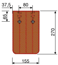
Firstbiber 15,5/27 Berliner Biber
